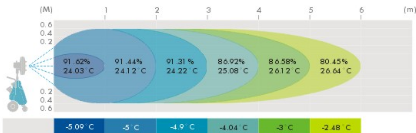
3-speed, variable pitch oscillating fan.
